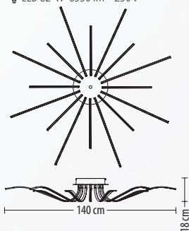
5330 PL-16 Q LED 82 W 6550 lm* 230V
