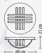
5471 PL-6 Q LED 54 W 4150 lm* 230 V
