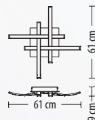
5303 PL-4 Q LED 35 W 2680 lm* 230 V
