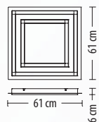
5369 PL-2 Q LED 59 W 3880 lm* 230 V
