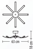
5585 PL-8 Q LED 35 W 2680 lm* 230 V
