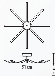
5584 PL-8 Q LED 57 W 4360 lm* 230 V
