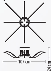
5259 PL-8 Q LED 35 W 2680 lm* 230 V
