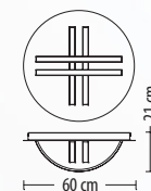
5474 PL-4 Q LED 36 W 2770 lm* 230 V
