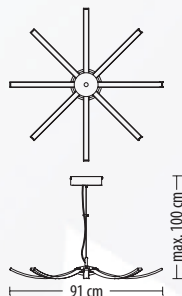
5580 Z-8 Q LED 57 W 4360 lm* 230 V
