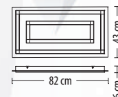
5367 PL-2 Q LED 59 W 3880 lm* 230 V
