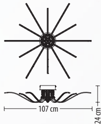
5257 PL-12 Q LED 52 W 4030 lm* 230 V
