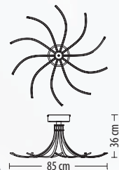
5450 Z-10 Q LED 50 W 3780 lm* 230 V
