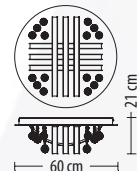
5470 PL-6 Q LED 54 W 4150 lm* 230 V
