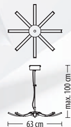
5581 Z-8 Q LED 35 W 2680 lm* 230 V
